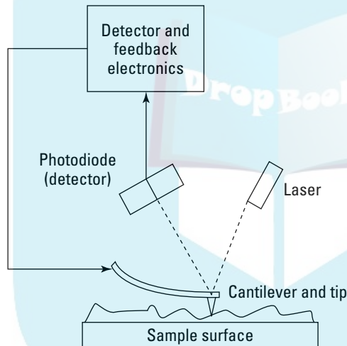
Figure 3-6: In an AFM, the small tip moves over the material surface.
